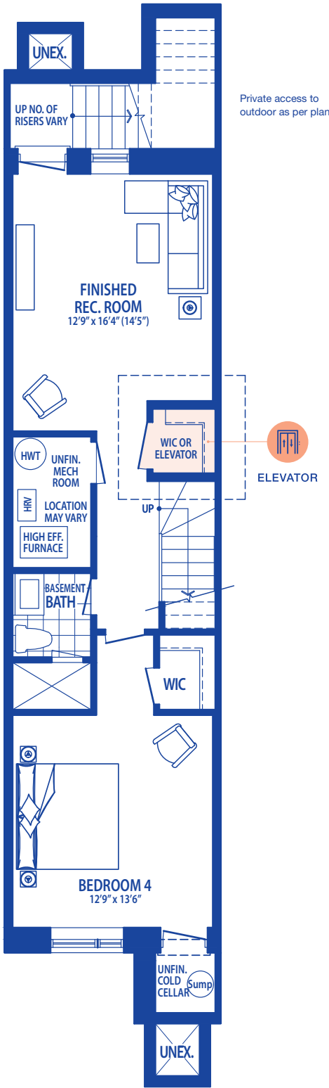
Basement
