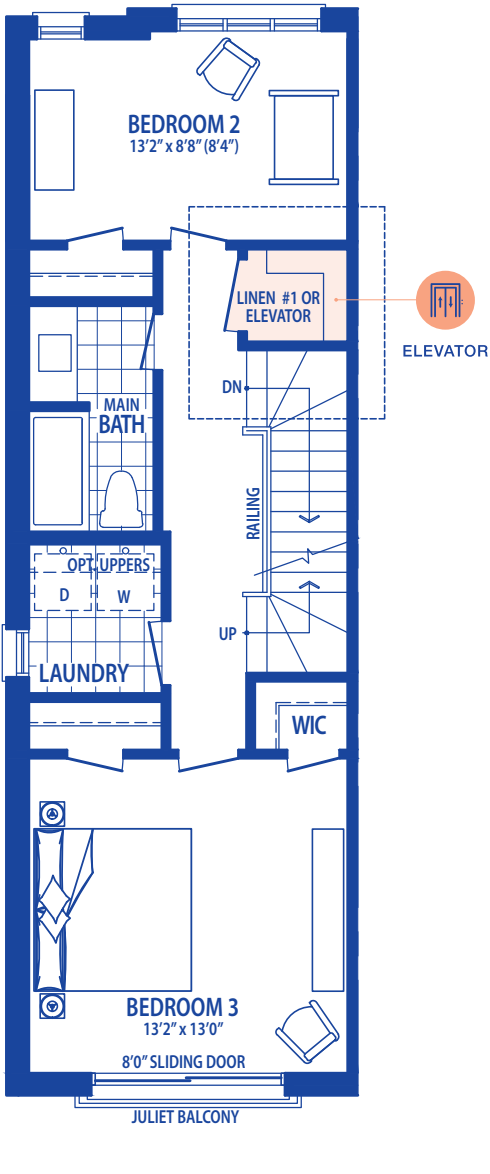
Second Level
